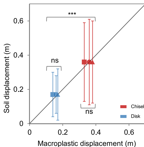
Fig. 4. Scatter plot of macroplastic and soil displacement (mean \pm SD) per tillage pass for small, large, and medium macroplastic sizes (differentiated in the three different shapes of scatter points, respectively) for chisel plow plots (dark red) and disk plow plots (blue). Standard deviation was presented in error bars. Stars indicate the significance level of the difference between means (ns: p-value > 0.05, ***: p-value < 0.0001).
